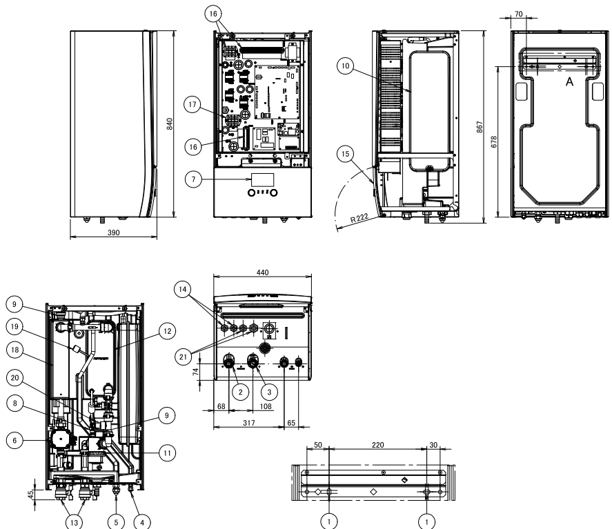
DETAIL A WALL FIXATION
